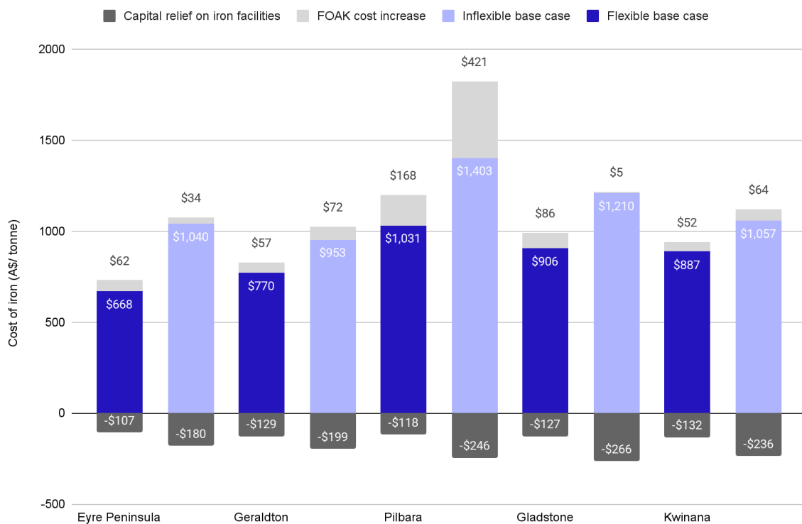
Figure 27: Impact of capital cost relief on the cost of iron in different locations, compared to estimated first-of-a-kind (FOAK) costs in each location
